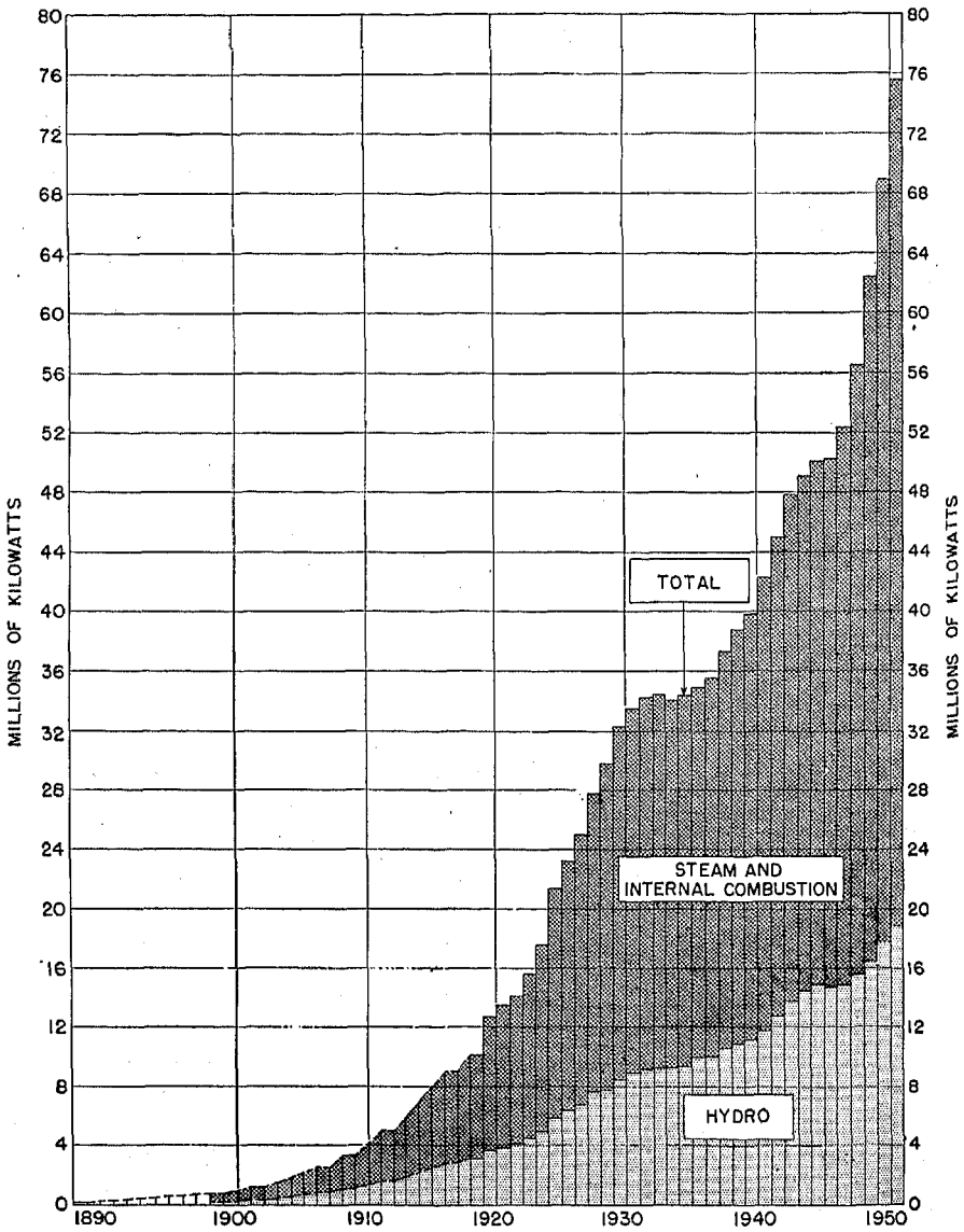
FIG. XXIII.—INSTALLED CAPACITY OF ELECTRIC UTILITY GENERATING PLANTS IN THE UNITED STATES: 1889 TO 1951
