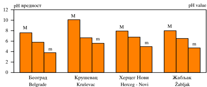
Граф. 2.5. ХЕМИЗАМ ПАДАВИНА, 2002. CHEMICAL COMPOSITION OF PRECIPITATION WATER, 2002
