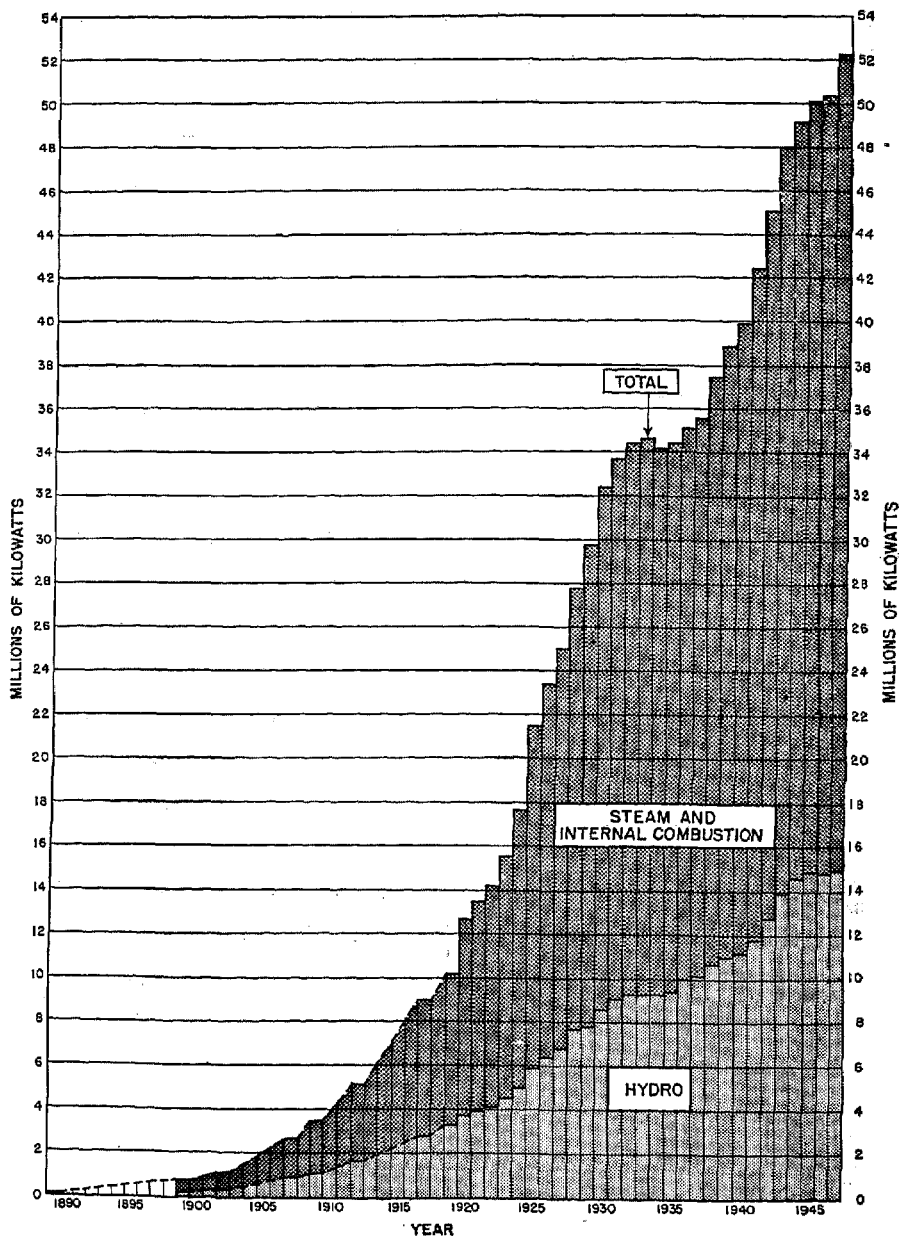
FIGURE Q.—INSTALLED CAPACITY OF ELECTRIC UTILITY GENERATING PLANTS IN THE UNITED STATES: 1889 TO 1947
